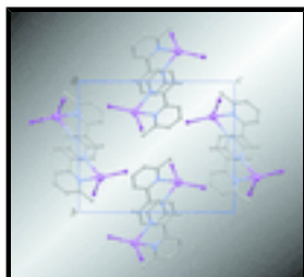
Fig. 2. Packing diagram for the crystal of the title compound viewed along the a axis.
